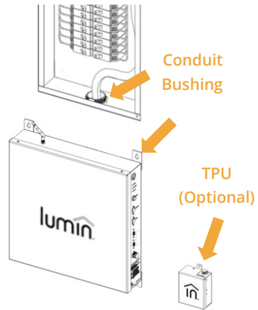
Flush-mounted installation
