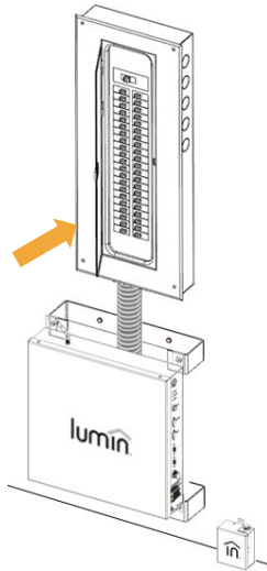
Surface-mounted installation
