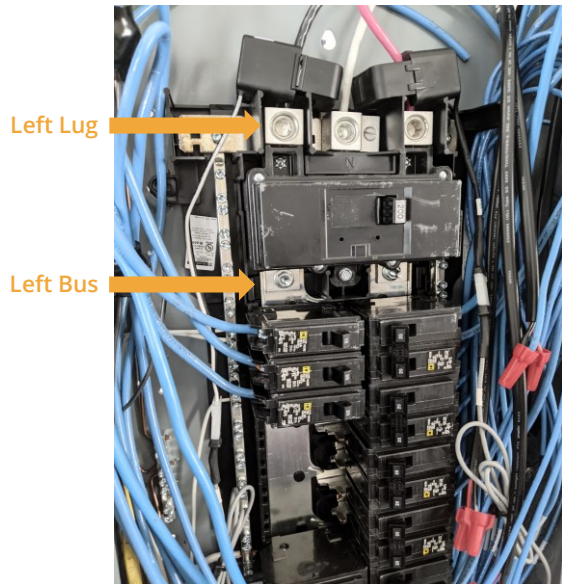
Figure C – Typical Main Breaker Electrical Panel
