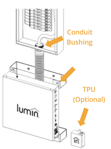
Surface-mounted installation
