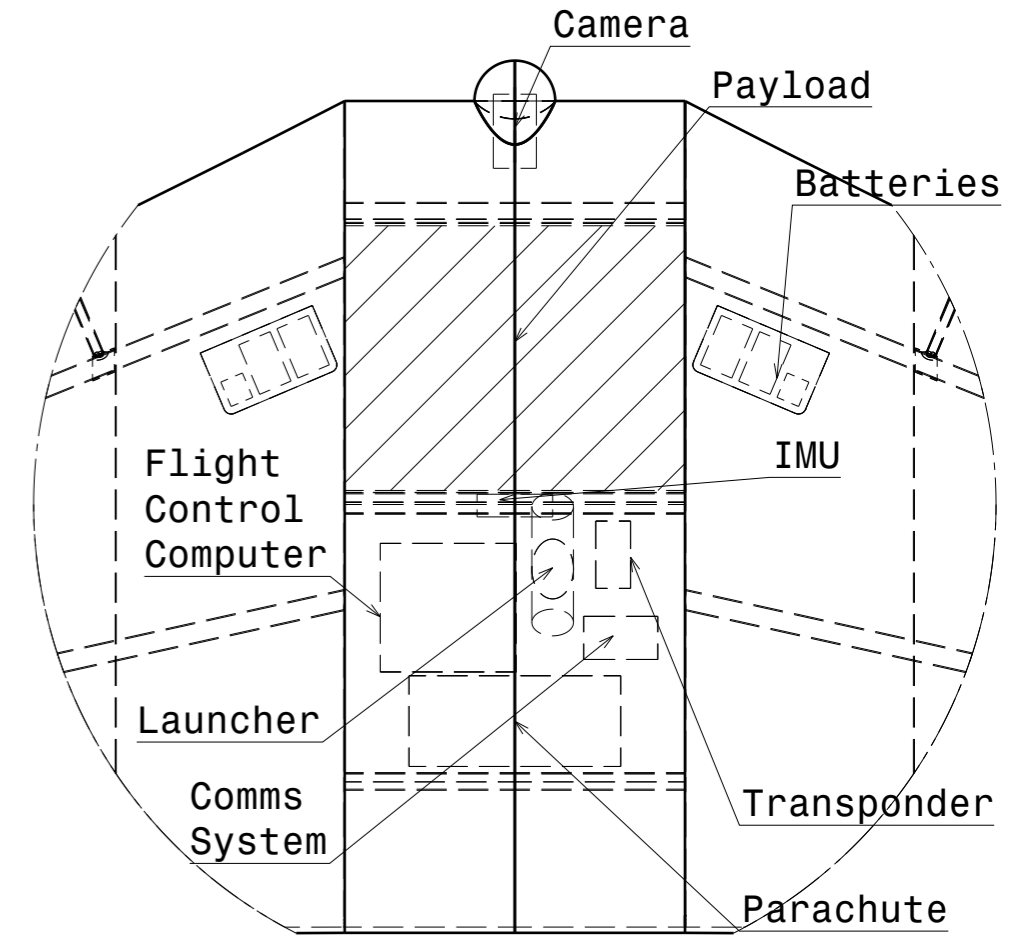
Detail A Payload Bay Scale: 1:10
