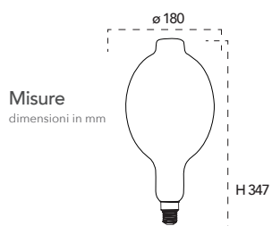
Lampada LED decorativa 8W 230V NDLS
