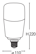
E27LB 32W Lampada LED LOWBAY classe A+
