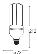
E27LB 27W Lampada LED LOWBAY classe A+
