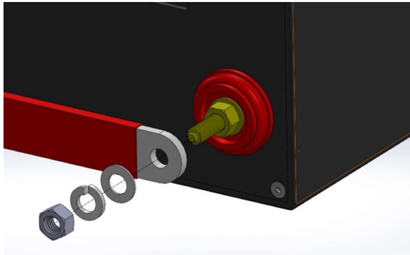
Figure 9.0 - Interconnecting Busbar Placement on PHI Battery Threaded Stud
