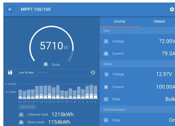
Screenshot of the VictronConnect app, showing real-time data and historical data.
