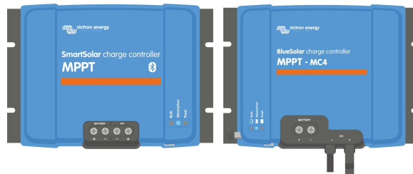
From left to right: Example of solar chargers with screw terminals and MC4 PV connections
