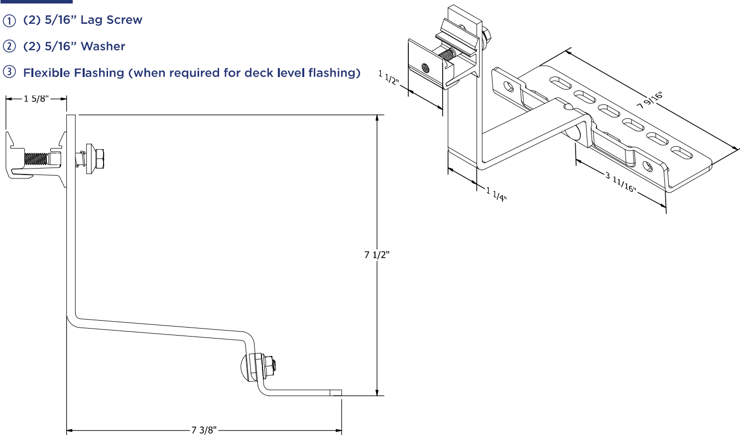
Dimensioned Ultra Rail Adjustable Tile Hook Assembly
