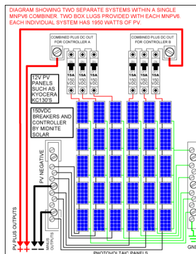
MNPV6 With circuit breakers
