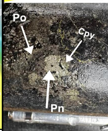
Ni sulphide blebs in hole 41
