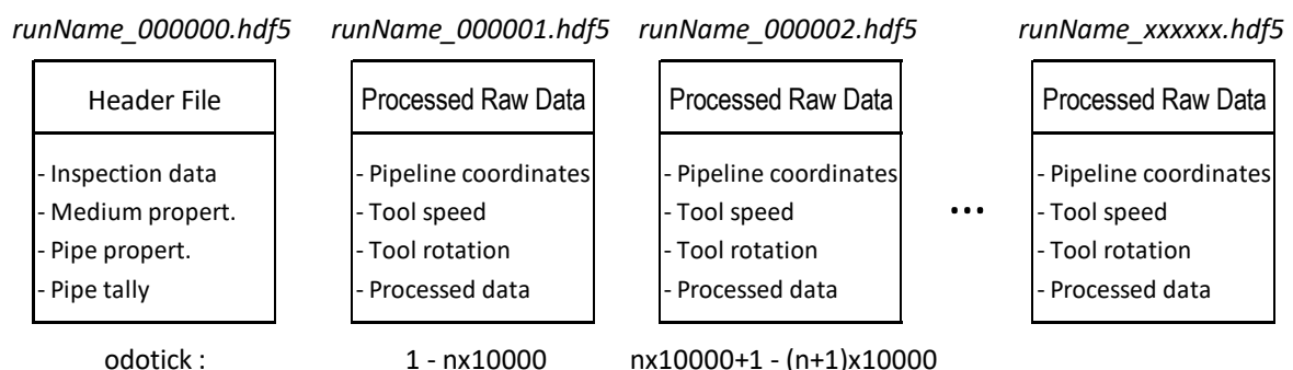
Figure 1: Data file structure
