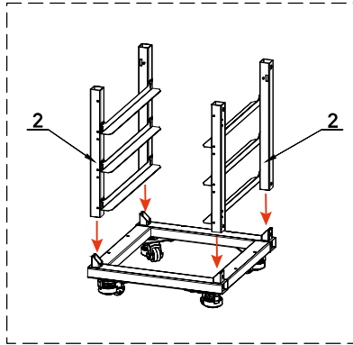
Align side racks to the bottom rack according to picture illustrated.
