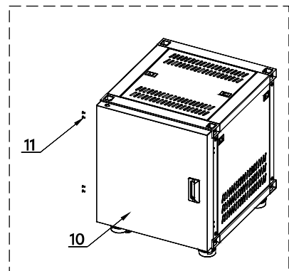
Install the symmetrical structured door to cabinet with KM5 screws
