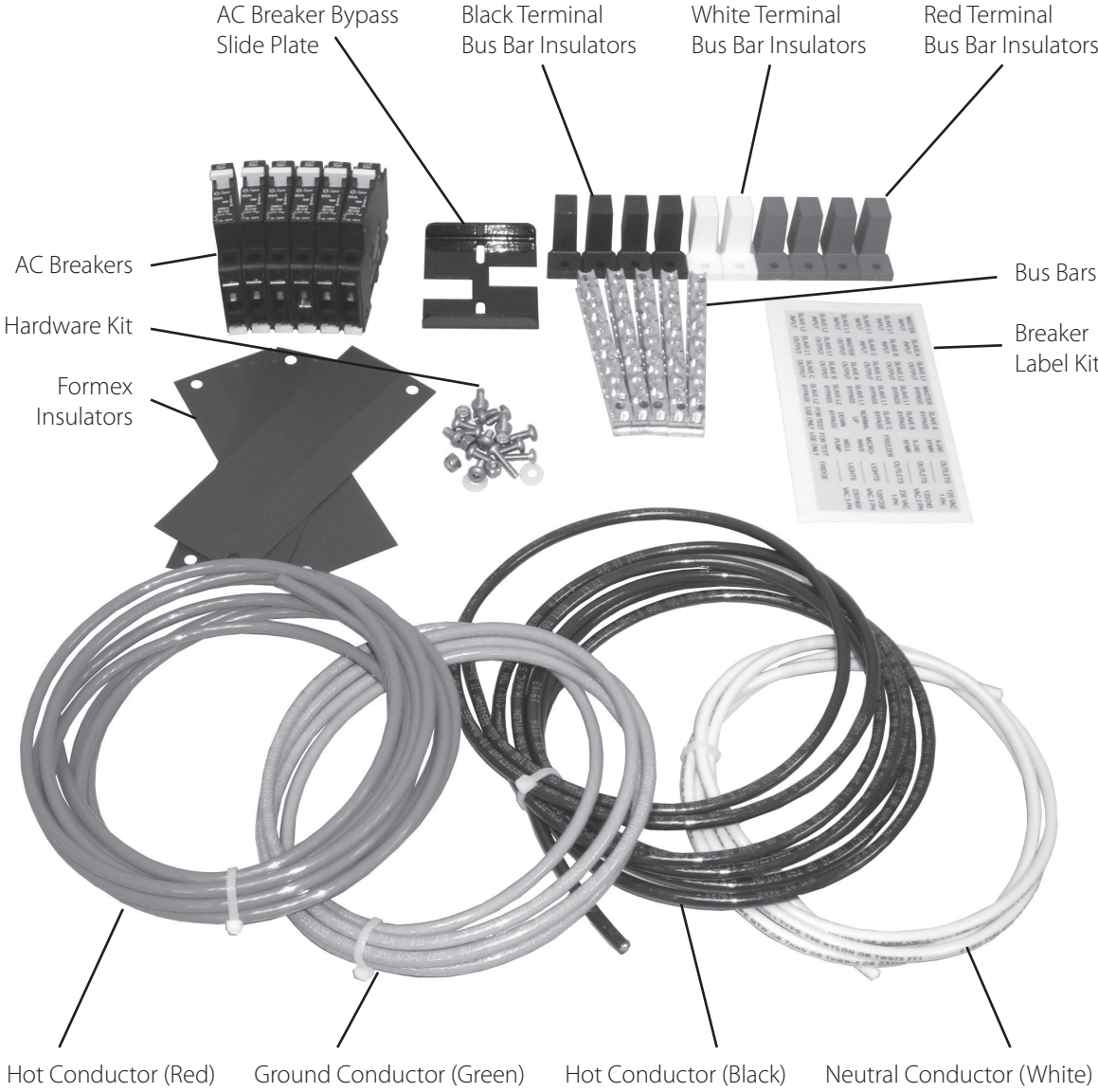
Figure 1: FW-IOB-D-120/240VAC
