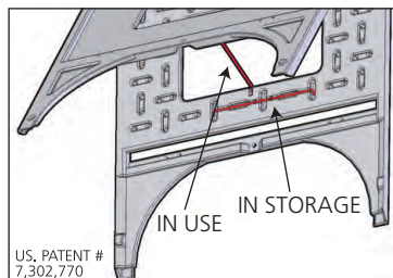
STABILIZING BRACE
