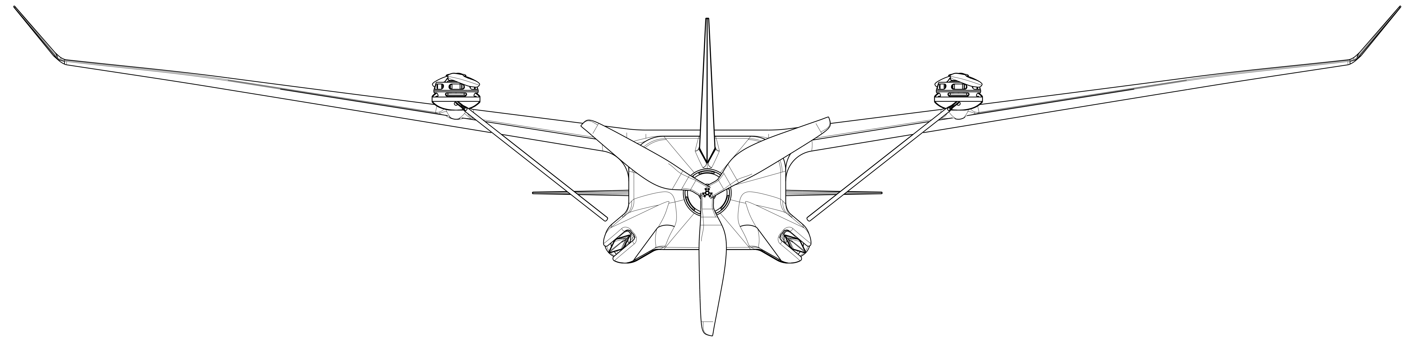
REAR VIEW Scale: 1:5
