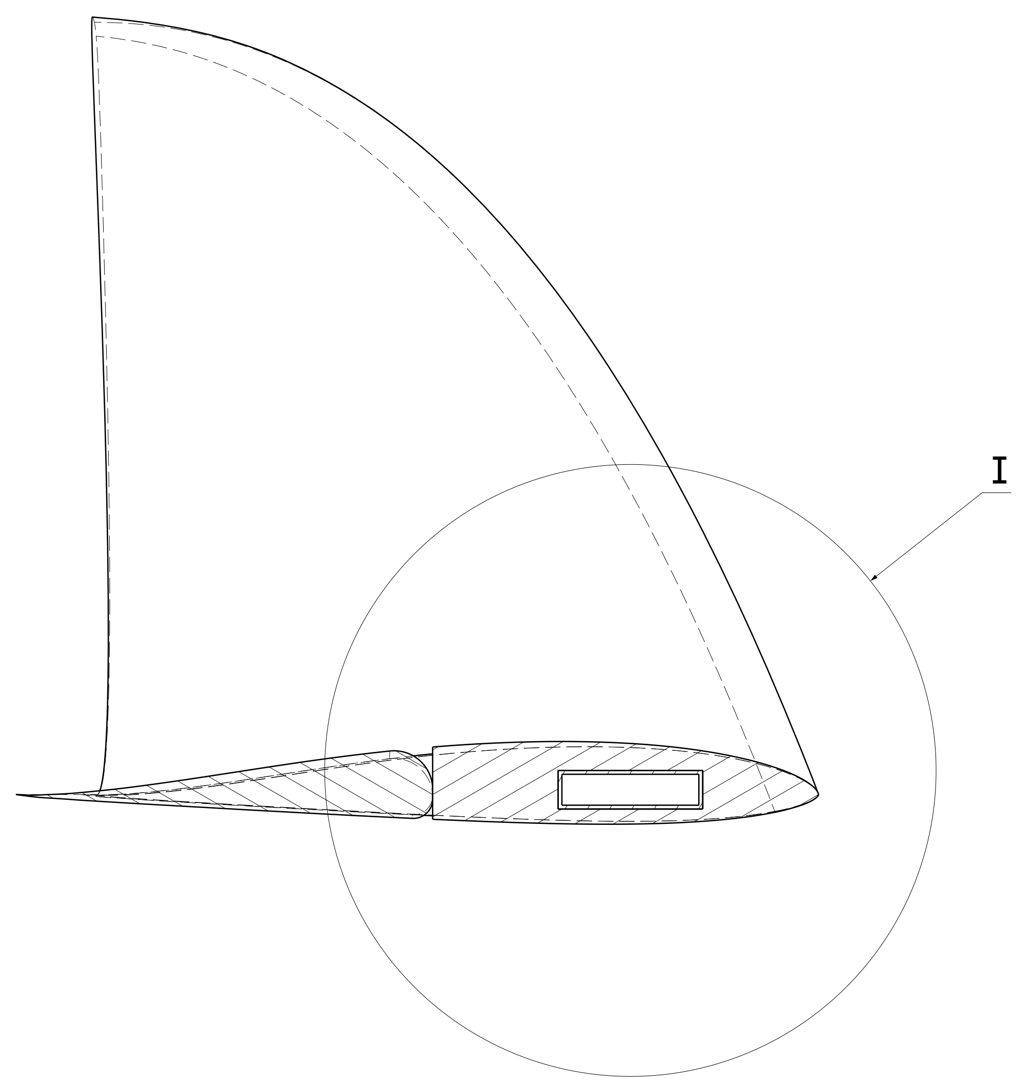
SECTION H-H
