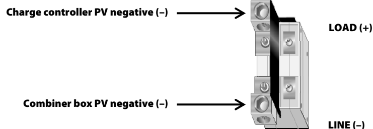
Figure 8 Positive-Grounded RTB
