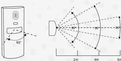
PIR Horizontal Detection Range Diagram
