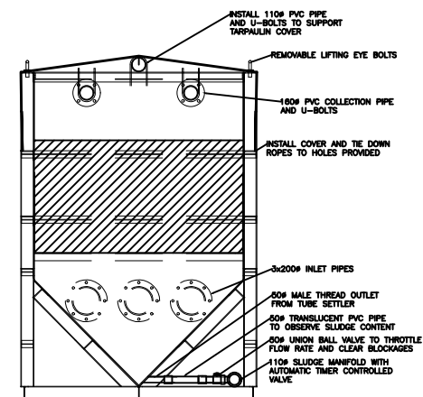
TRANSVERSE SECTION
