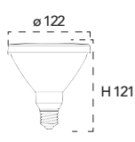
Lampadina a Led 18W, 240V
