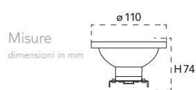
Lampadina a Led 13W, AC/DC 12V
