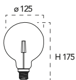
Lampadina a Led 16W, 240V
